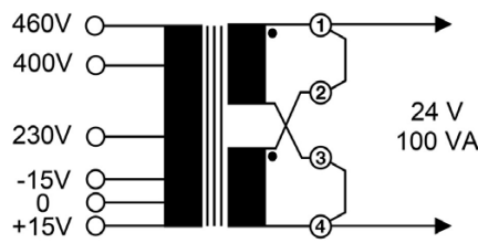
PARALLEL CONNECTION
